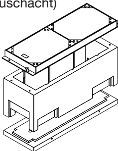
P-Schacht VI - 120/40/60 cm i.L.
