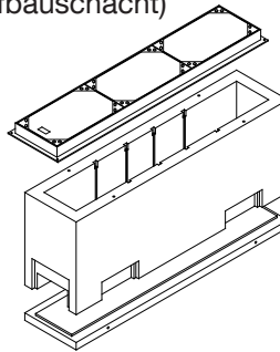
P-Schacht III - 80/40/70 cm i.L.
