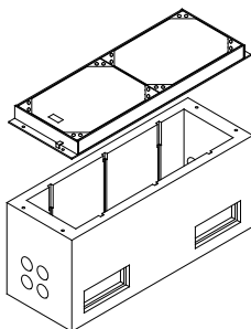
P-Schacht VI - 120/40/60 cm i.L.
